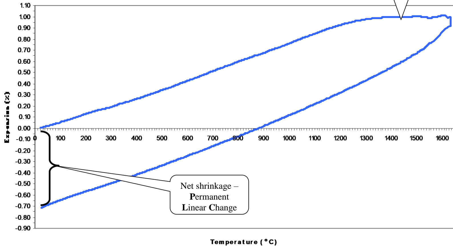
Typical Reversible Thermal Expansion Plot
